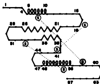
Turtle Egg White Inhibitor (14% \alpha , 25% \beta )
