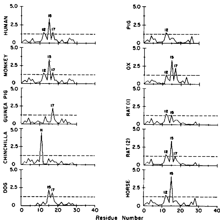
FIGURE 1 Probability of \beta -turn occurrence in C-peptides of proinsulin in 10 mammalian species. The dashed horizontal lines correspond to an arbitrary cutoff value of p_i = 1.25 \times 10^{-4} . The numbered probability peaks were predicted as \beta -turns.
