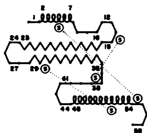
Snoil Inhibitor K (14% \alpha , 29% \beta )
